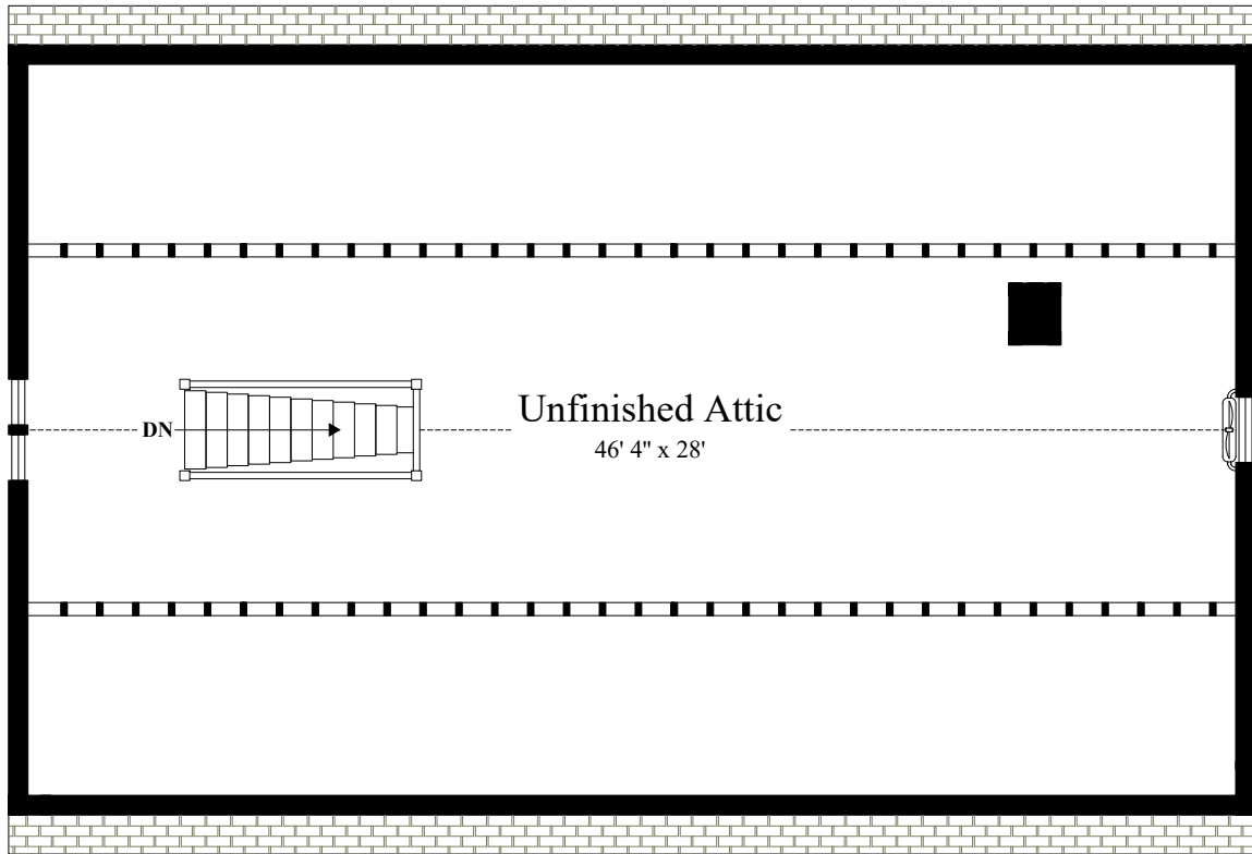
THIRD FLOOR (ceiling = 9' 2" to center beam)
