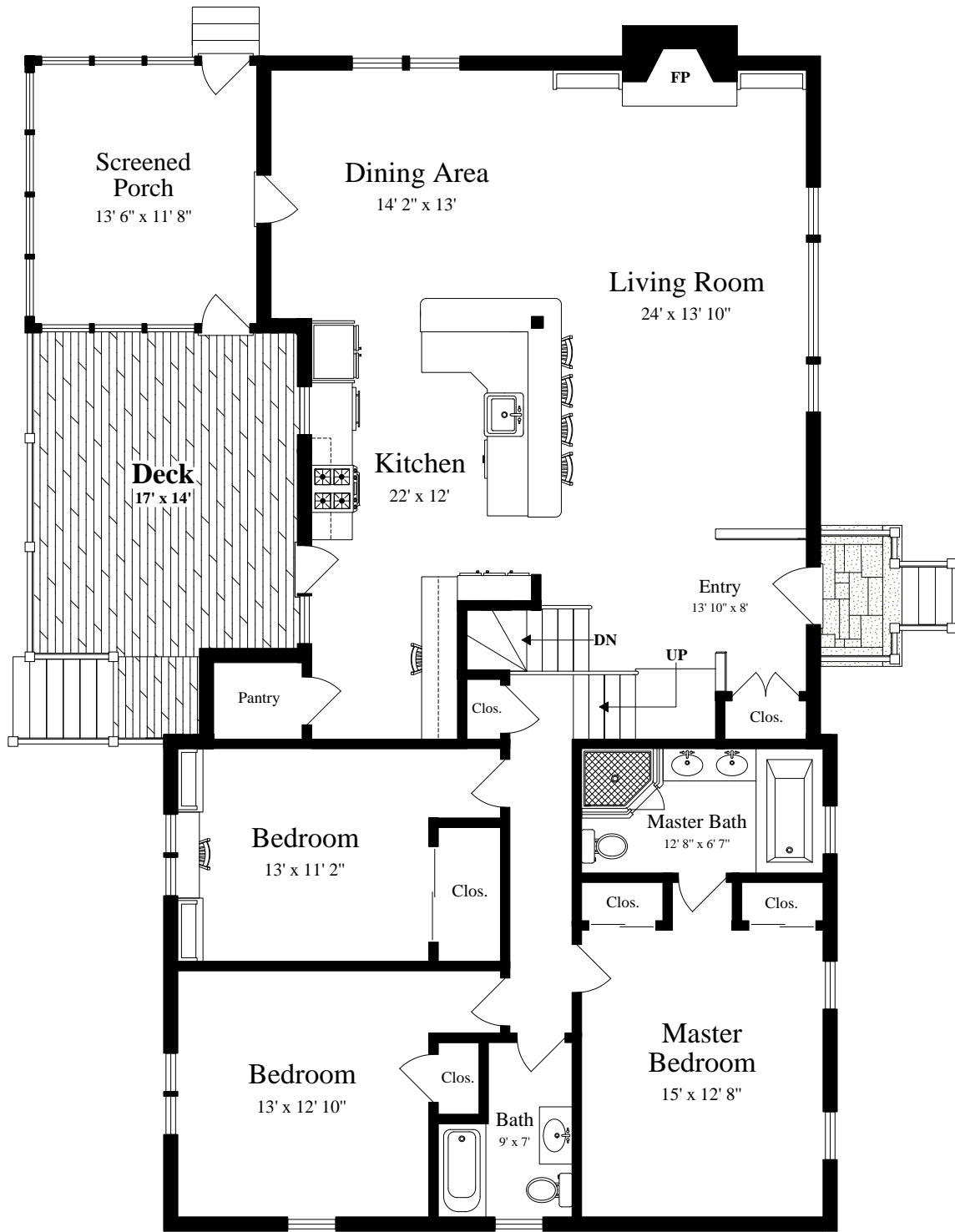
FIRST FLOOR (ceiling = 8')
