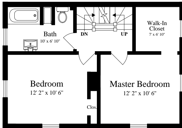
SECOND FLOOR (ceiling = 8')
