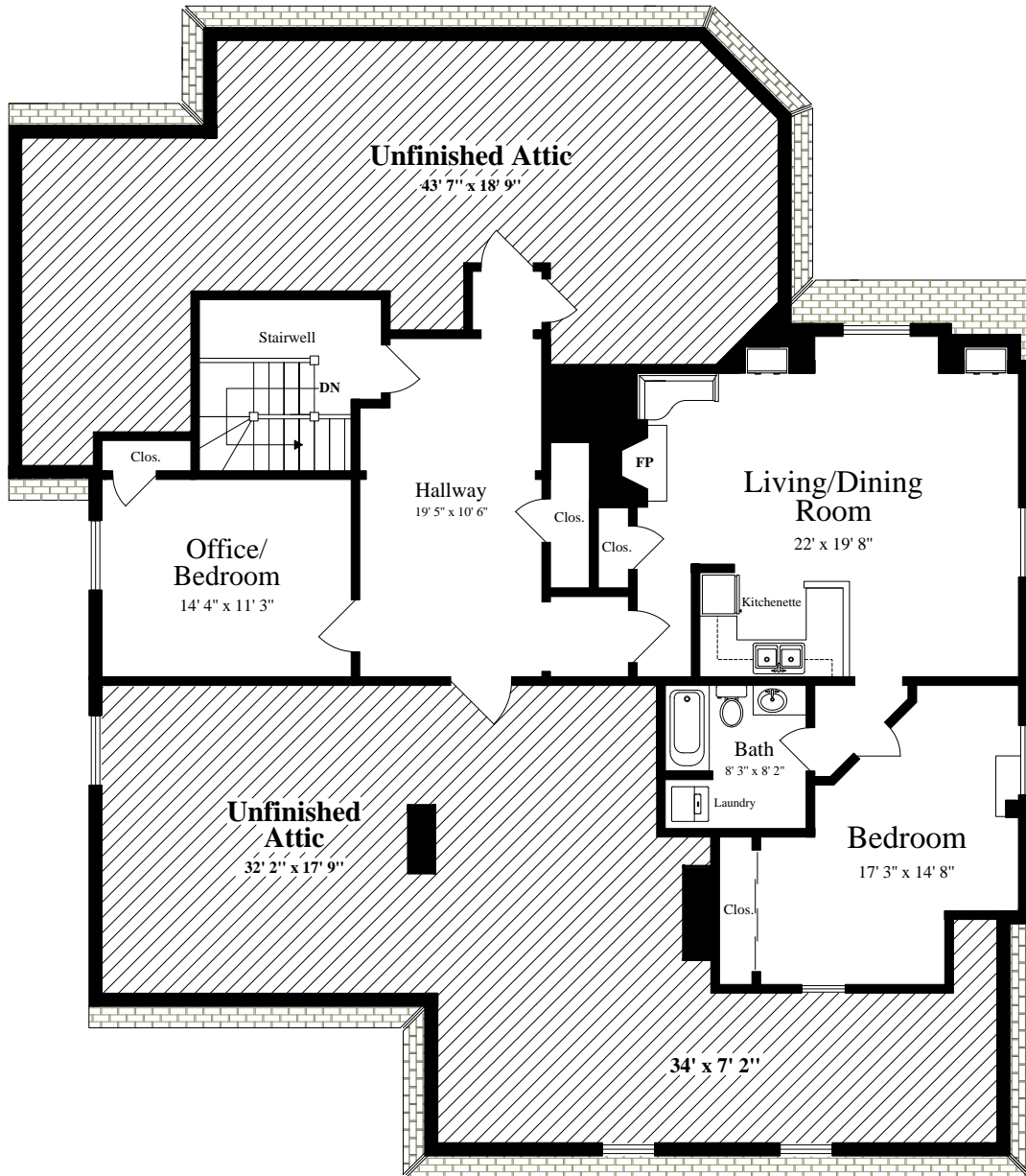
THIRD FLOOR (ceiling = 9')
