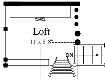
4th LEVEL (vaulted ceiling = 11' 2'')
