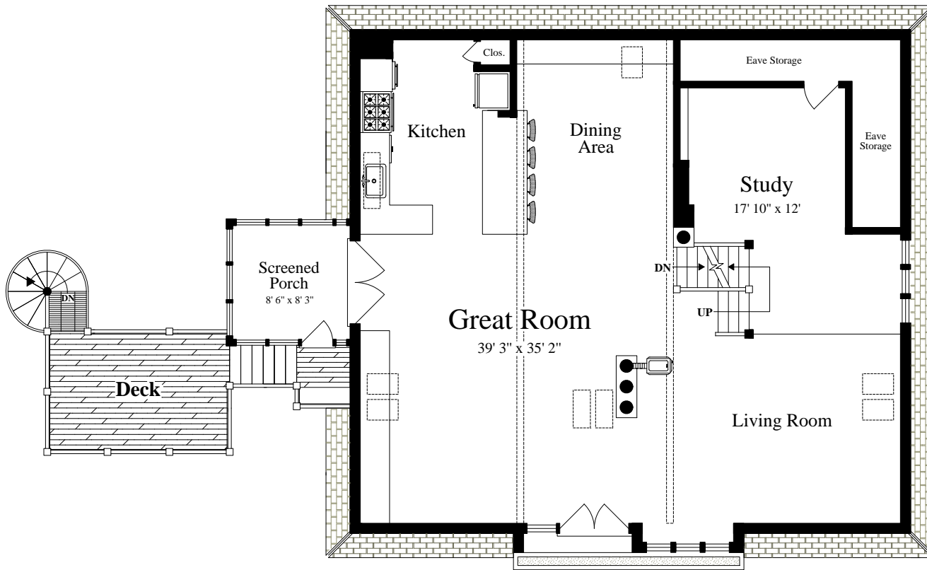
3rd LEVEL & MEZZANINE (vaulted ceiling = 19' 7'')
