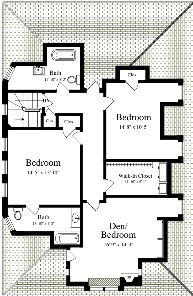
THIRD FLOOR (ceiling = 7' 10")
