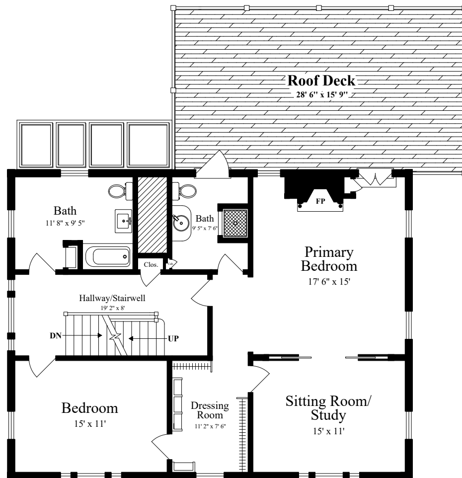
SECOND FLOOR (ceiling = 7' 5")
