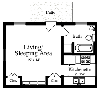
FIRST FLOOR - Guest House (vaulted ceiling = 14' 8")
