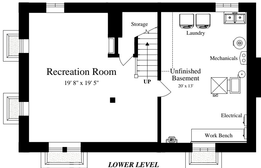
LOWER LEVEL (ceiling = 7' 9")
