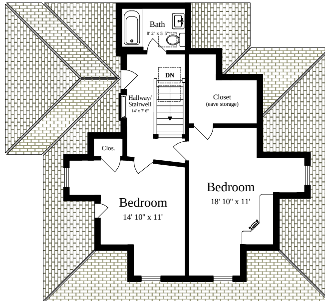
THIRD FLOOR (ceiling = 7' 3")
