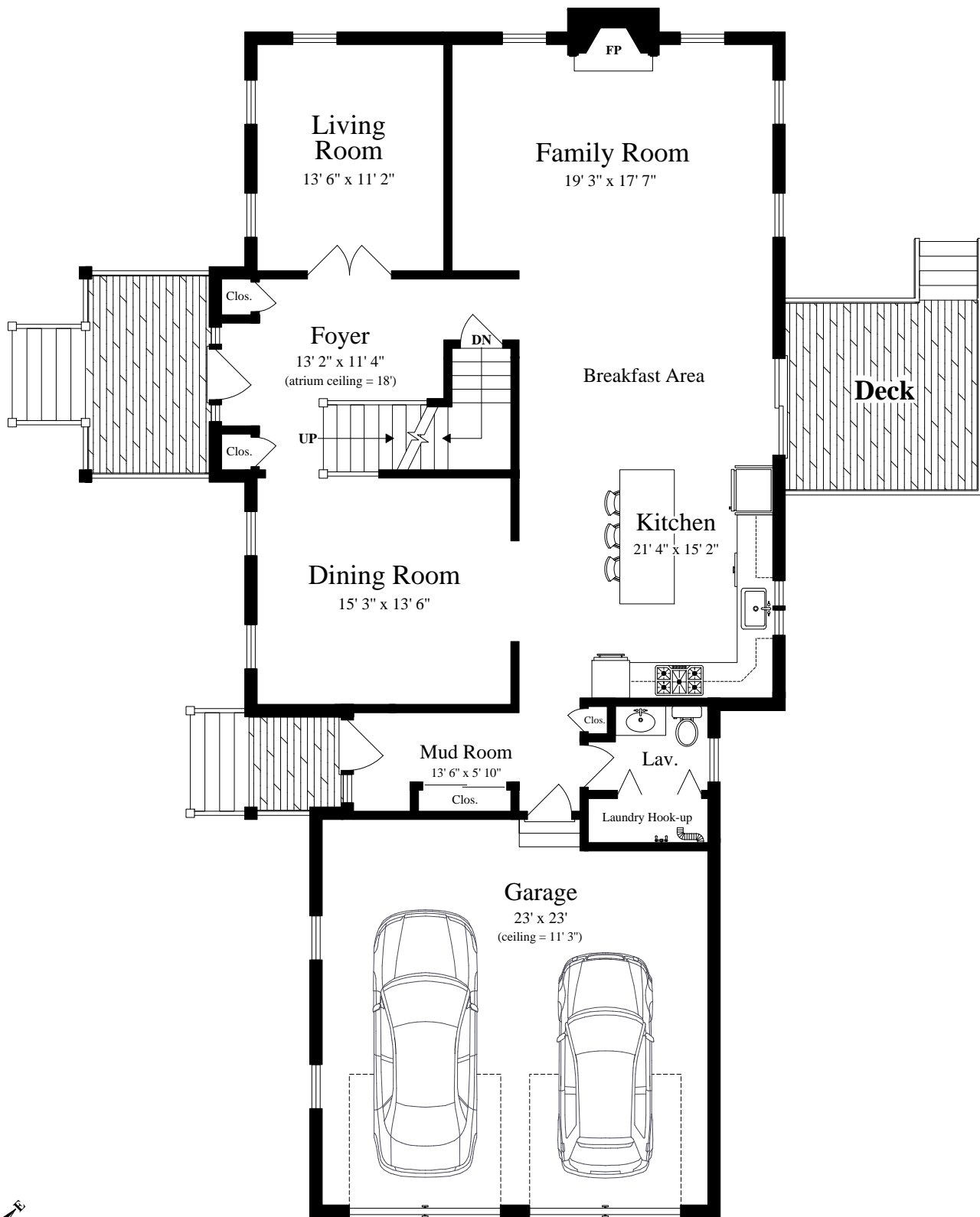
FIRST FLOOR (ceiling = 9')
