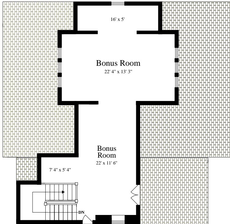
THIRD FLOOR (ceiling = 6' 9")
