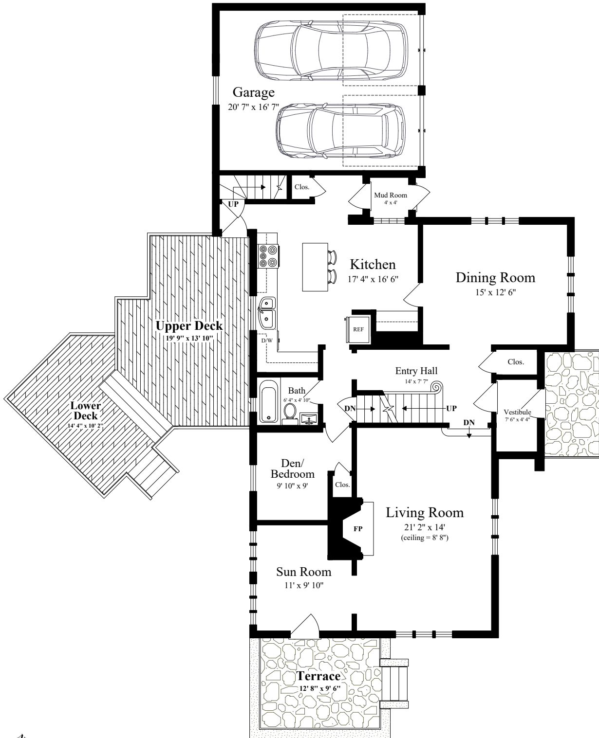
FIRST FLOOR (ceiling = 7' 9")
