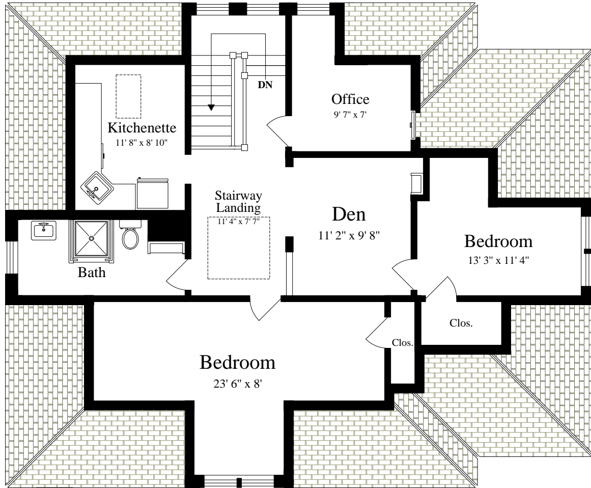
THIRD FLOOR (ceiling = 7' 6")
