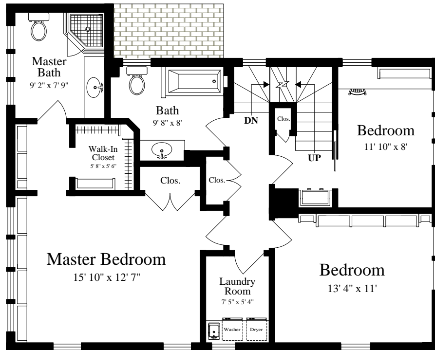
SECOND FLOOR (ceiling = 7' 10")
