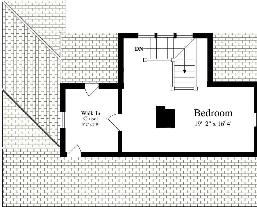
THIRD FLOOR (ceiling = 7' 2")
