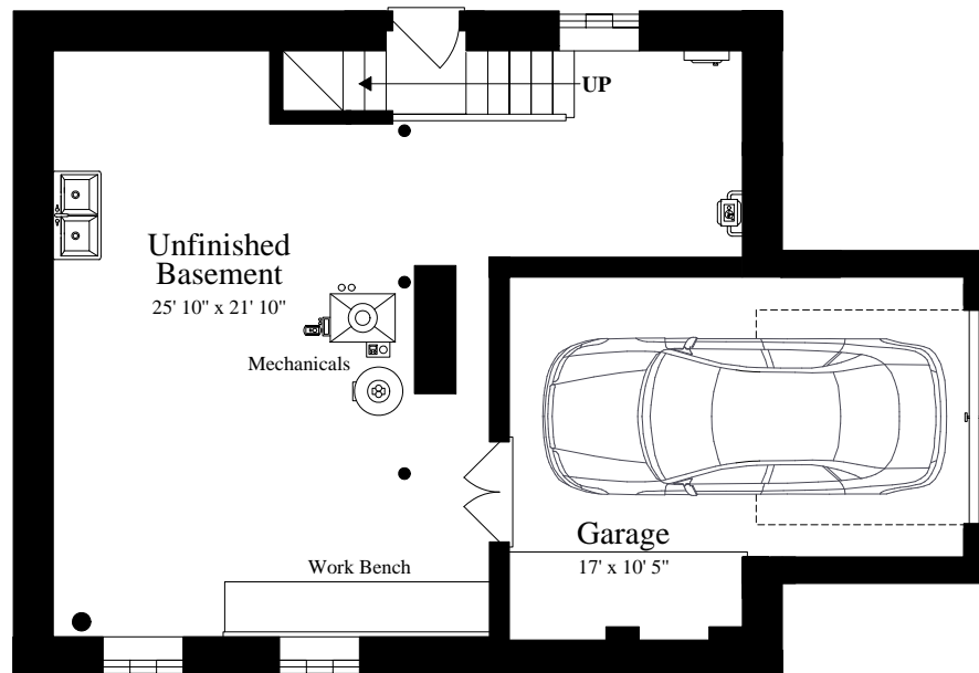
LOWER LEVEL (ceiling = 7')
