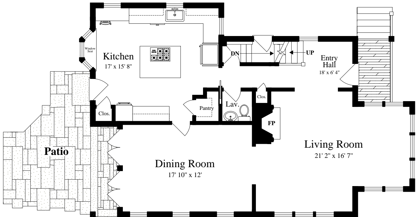
FIRST FLOOR (ceiling = 8')
