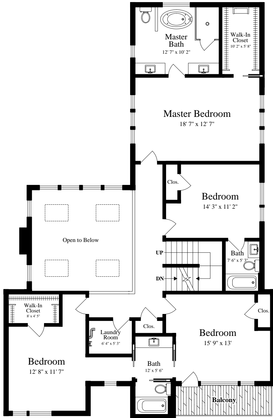
SECOND FLOOR (ceiling = 9')
