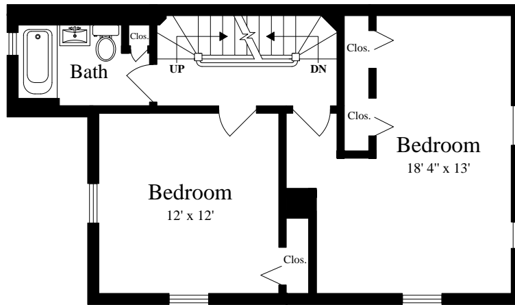
SECOND FLOOR (ceiling = 8' 6")
