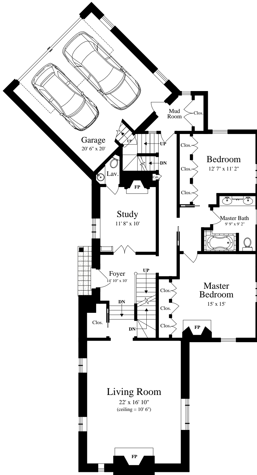
FIRST FLOOR (ceiling = 7' 7")
