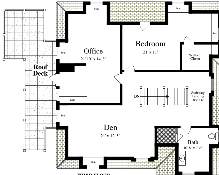
THIRD FLOOR (vaulted ceiling = 11')
