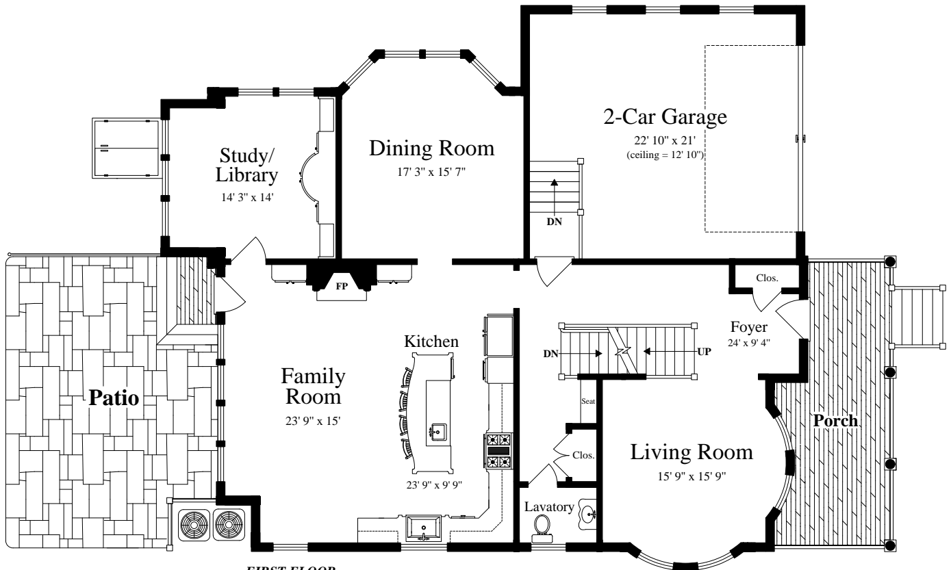
FIRST FLOOR (ceiling = 9' 5")
