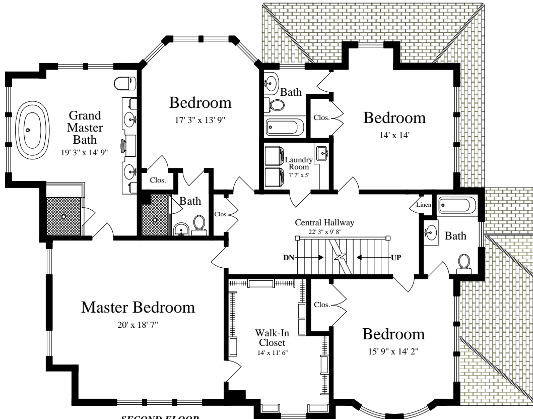
SECOND FLOOR (ceiling = 9')
