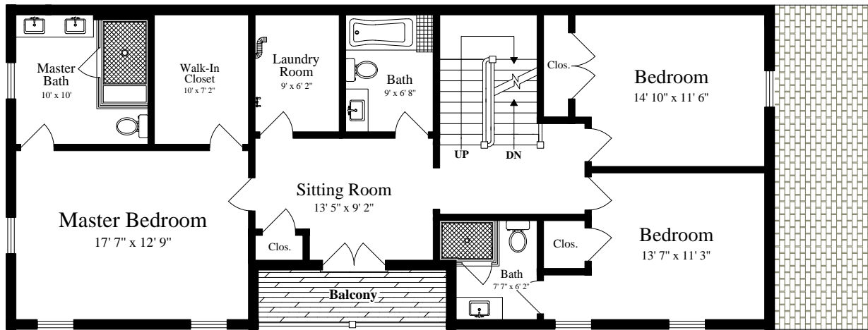
SECOND FLOOR (ceiling = 9')
