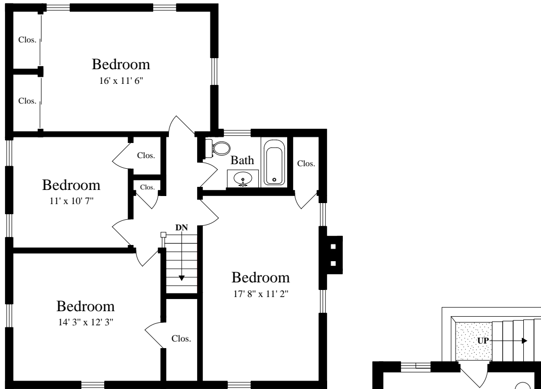
SECOND FLOOR (ceiling = 7')
