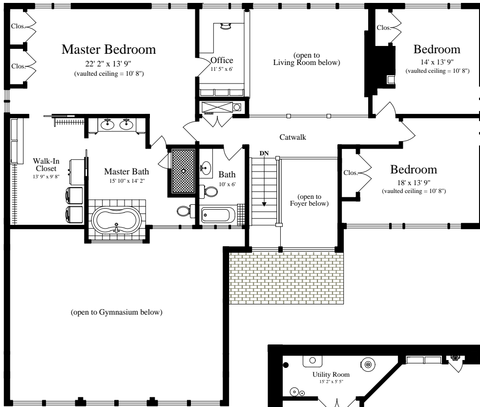
SECOND FLOOR (ceiling = 7' 10")
