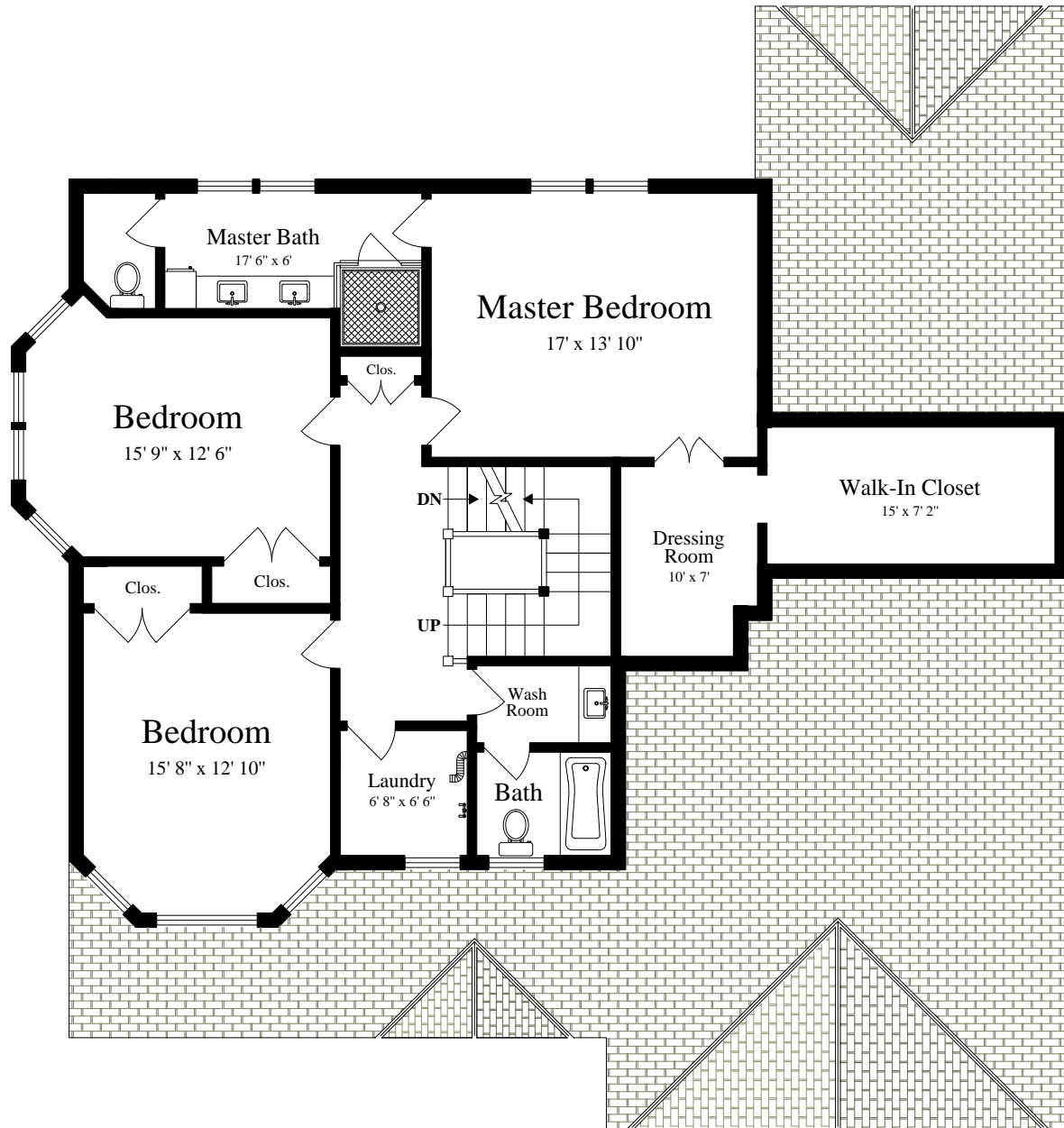
SECOND FLOOR (ceiling = 8' 6")
