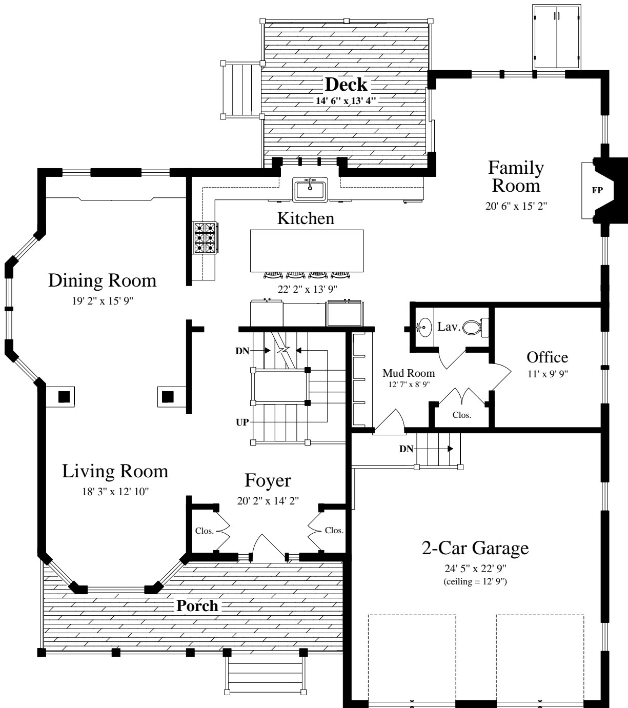
FIRST FLOOR (ceiling = 9')
