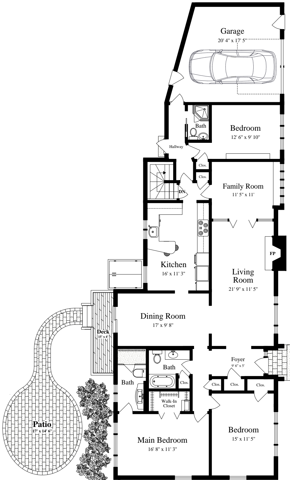
FIRST FLOOR
