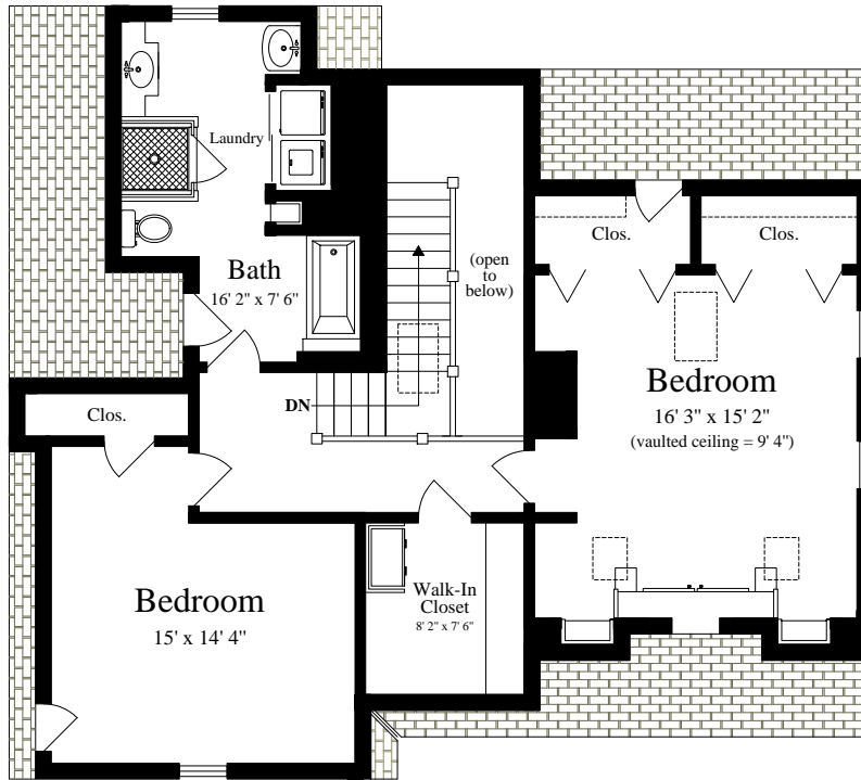
THIRD FLOOR (ceiling = 7')
