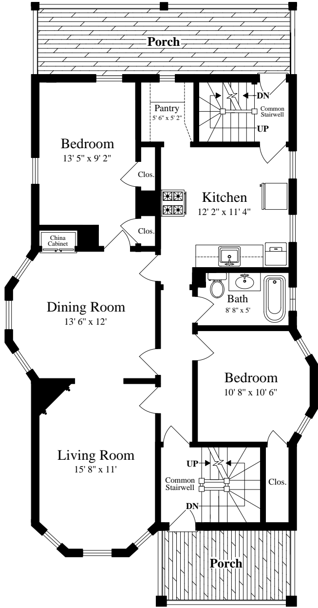
SECOND FLOOR/Apt. #2 (ceiling = 8' 8")
