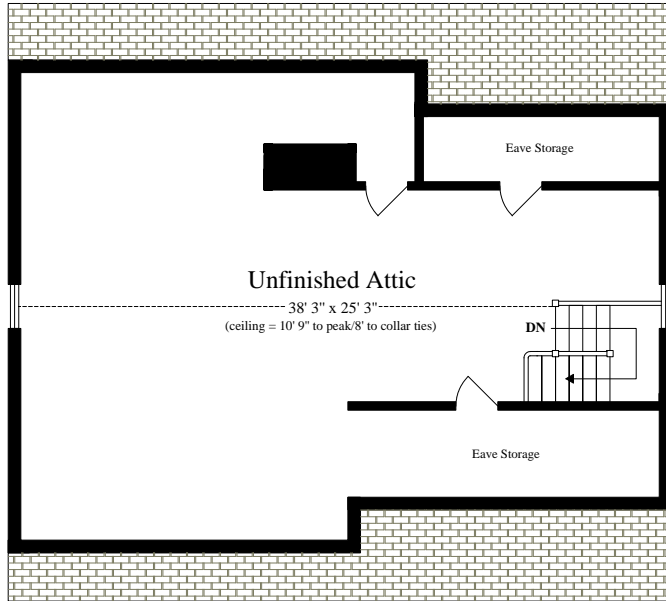
FOURTH FLOOR (ceiling = 8')
