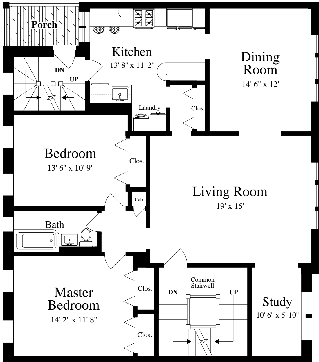
SECOND FLOOR (ceiling = 9')
