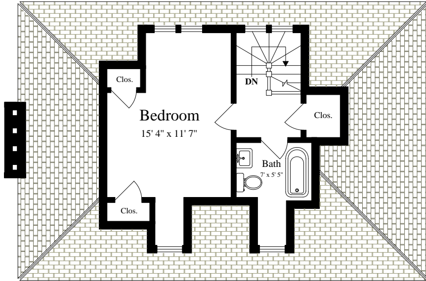
THIRD FLOOR
