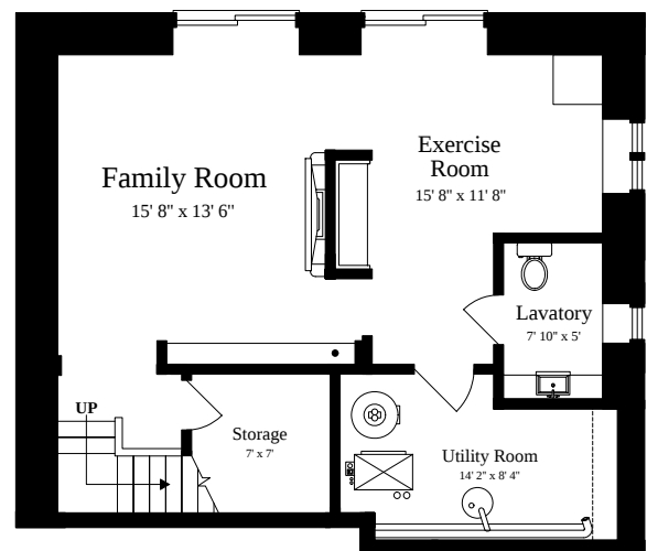
LOWER LEVEL (ceiling = 7' 7")
