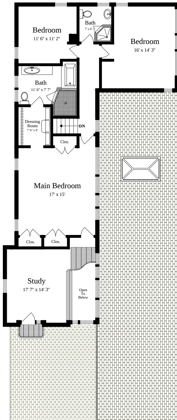
SECOND FLOOR (vaulted ceiling = 11')
