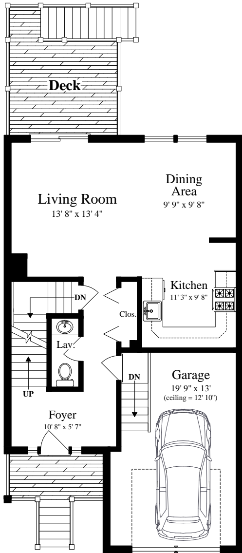
FIRST FLOOR (ceiling = 7' 10")
