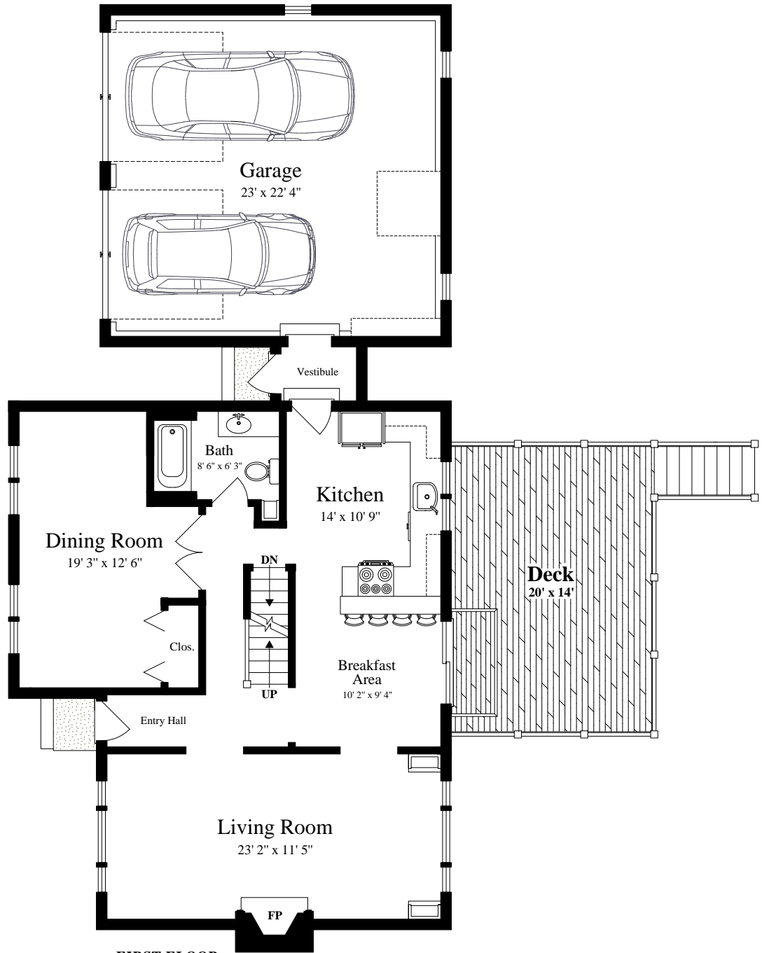
FIRST FLOOR (ceiling = 7' 2")
