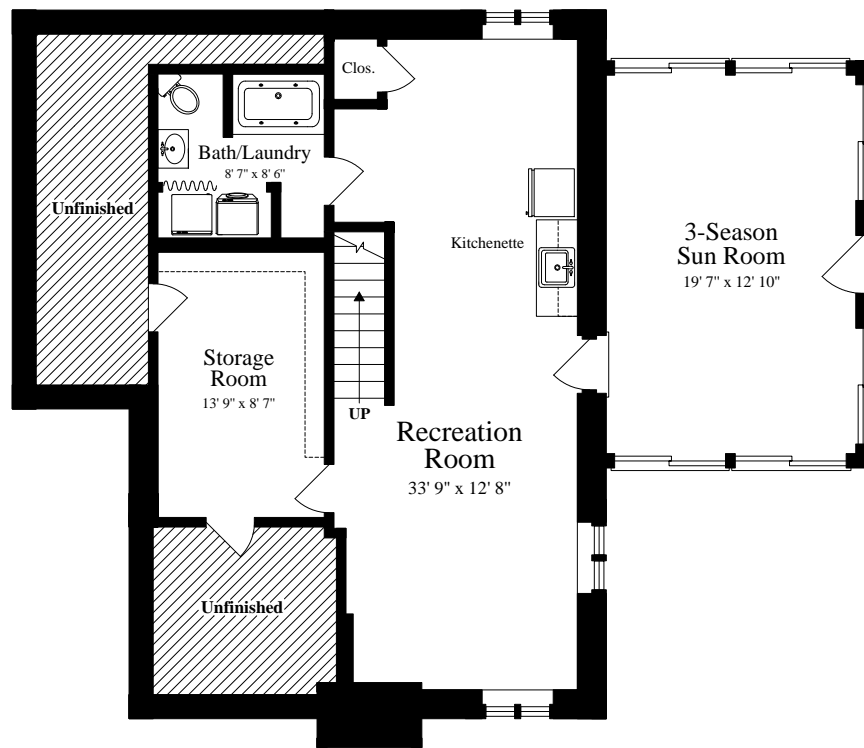
LOWER LEVEL (ceiling = 7')
