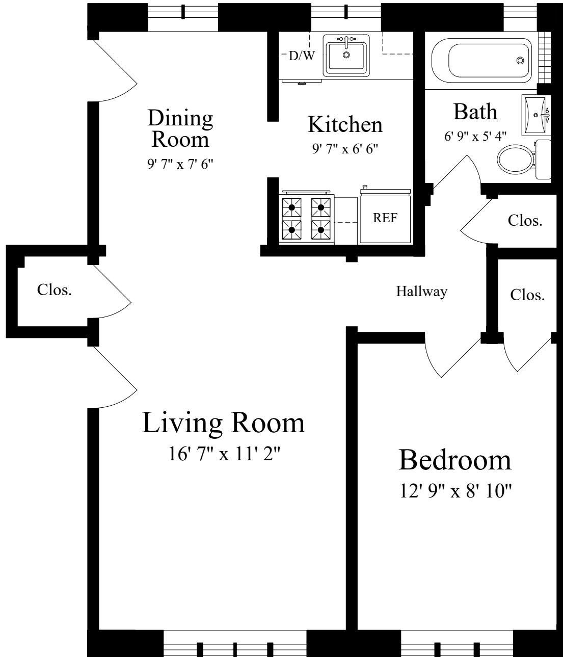
THIRD FLOOR (ceiling = 8')
