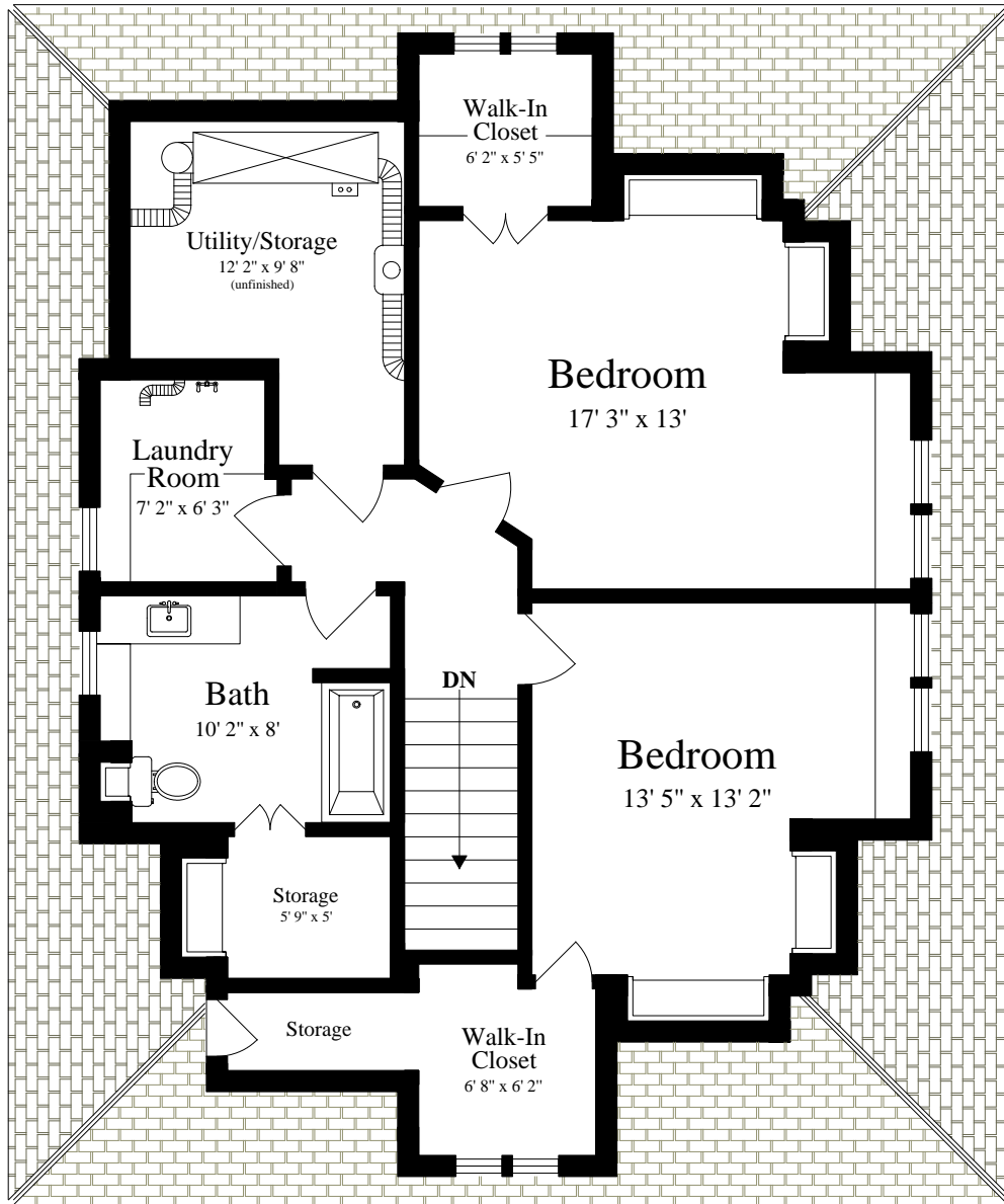
THIRD FLOOR (ceiling = 8')
