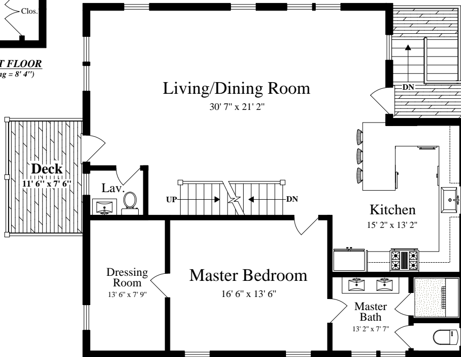
SECOND FLOOR (ceiling = 8' 2")
