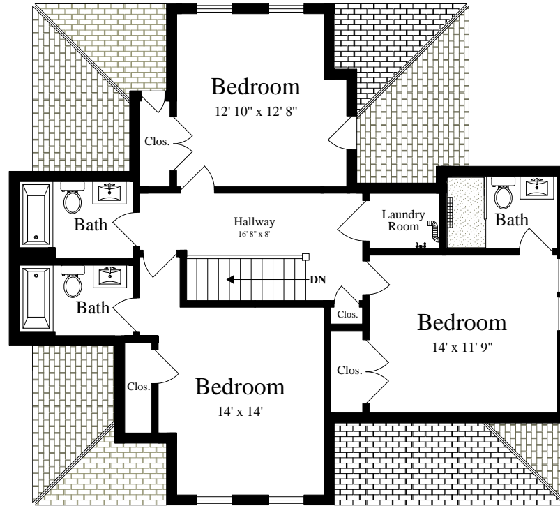
THIRD FLOOR (ceiling = 8')
