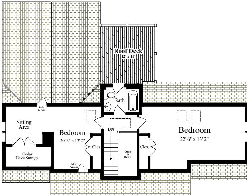
THIRD FLOOR (Cathedral ceiling = 9' 2")
