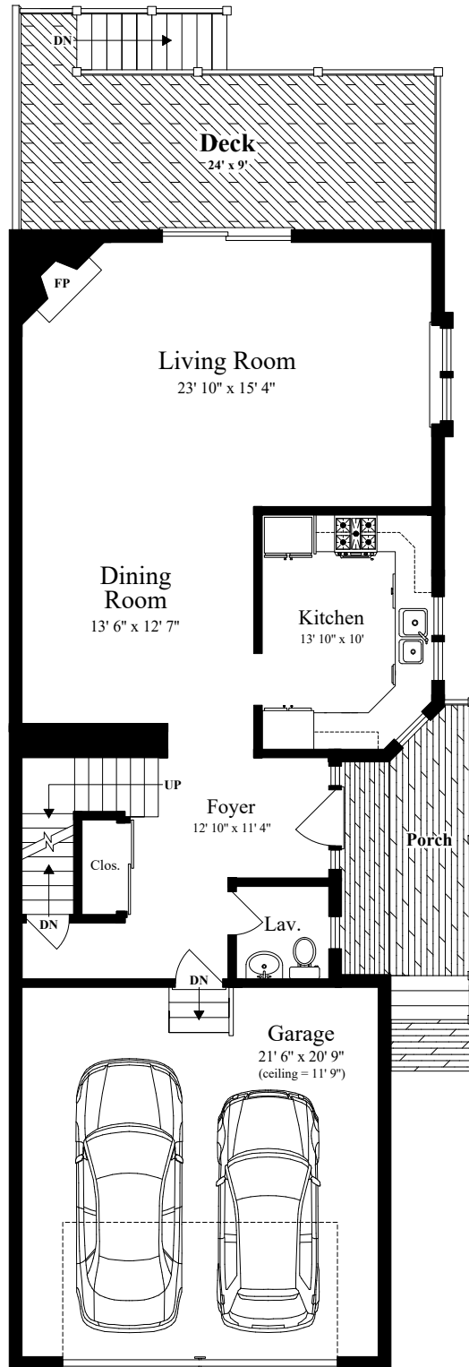
FIRST FLOOR (ceiling = 9')
