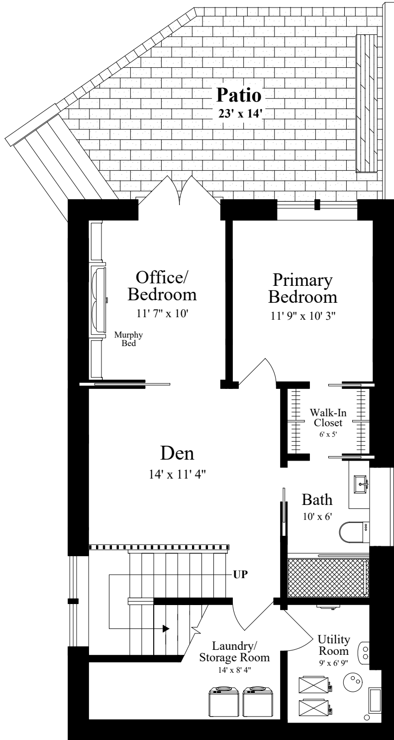
GROUND LEVEL (ceiling = 8' 9")
