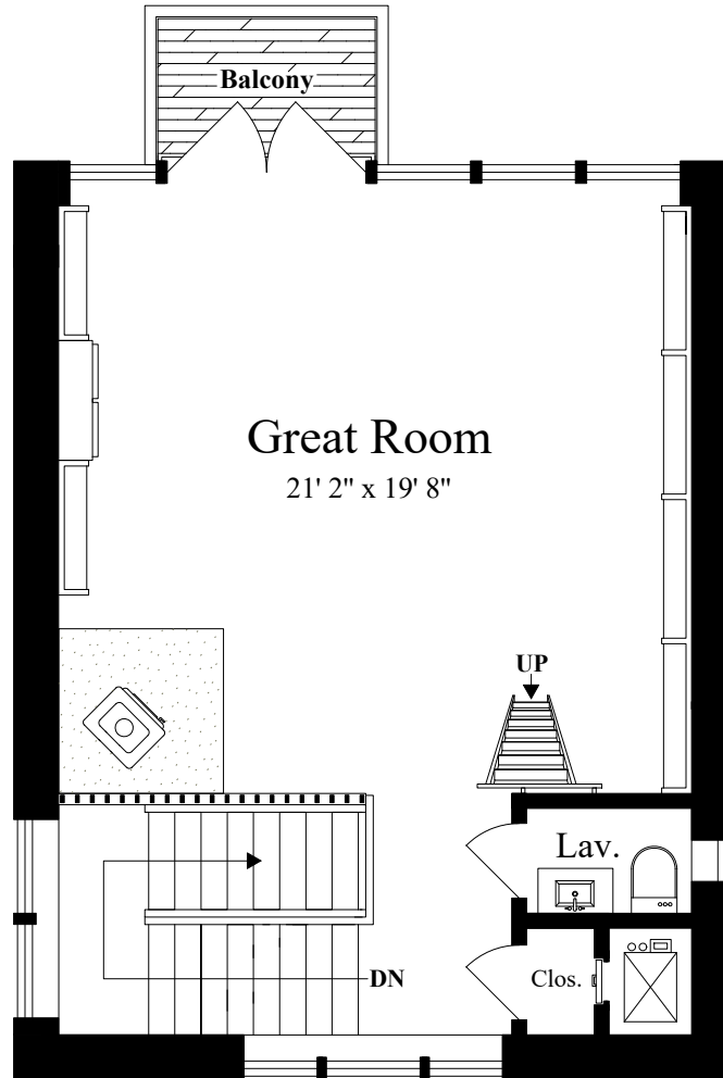
SECOND FLOOR (cathedral ceiling = 20' 10")
