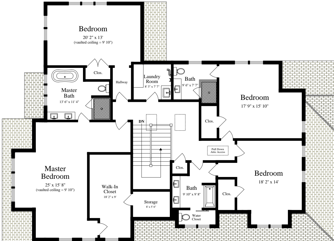
SECOND FLOOR (ceiling = 9')
