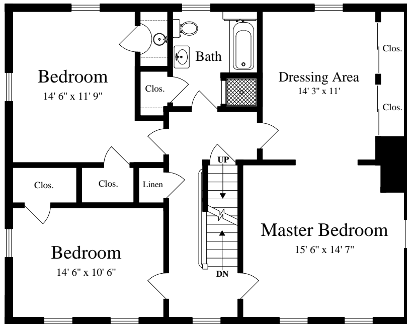
SECOND FLOOR (ceiling = 8' 6")
