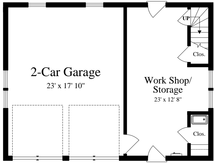
FIRST FLOOR (ceiling = 9')
