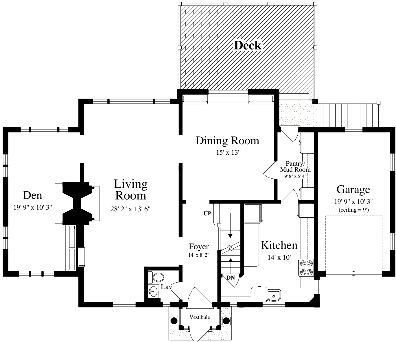
FIRST FLOOR (ceiling = 8' 4")
