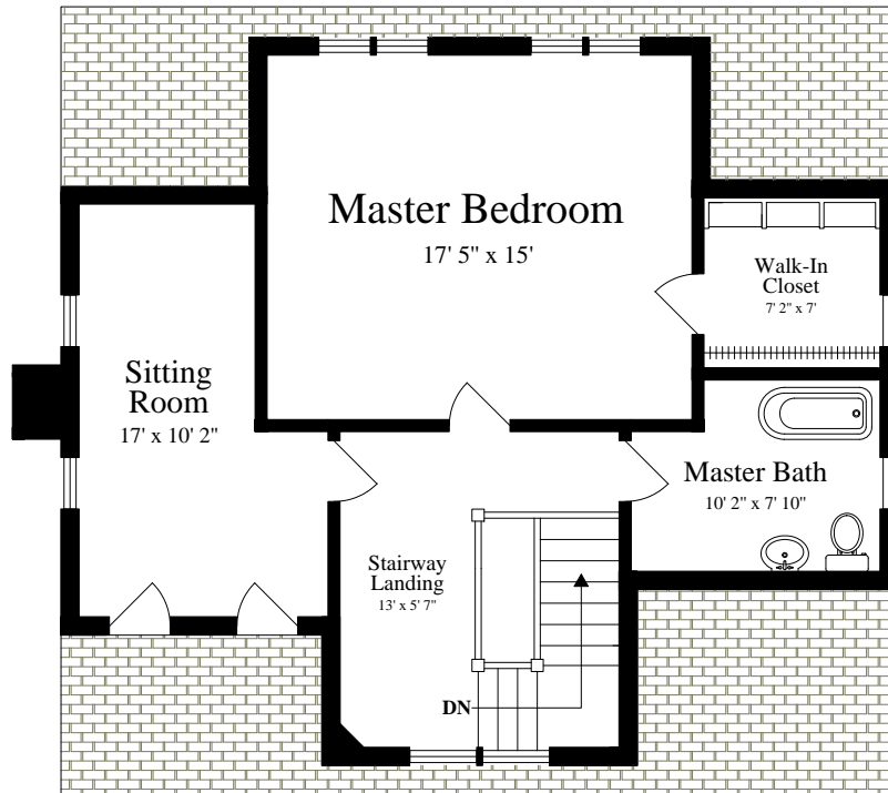
THIRD FLOOR (ceiling = 6' 10")
