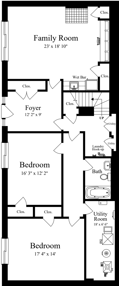
LOWER LEVEL (ceiling = 8')
