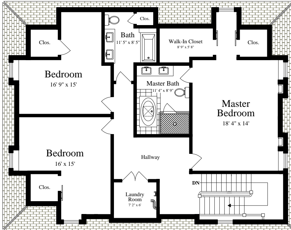
SECOND FLOOR (ceiling = 9')
