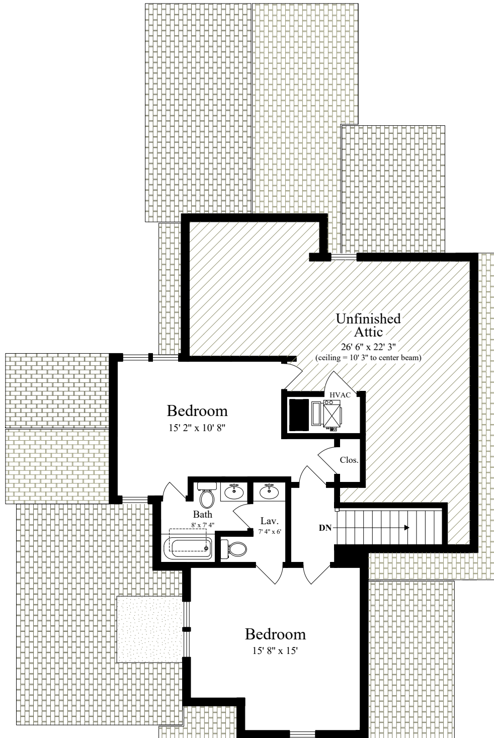
SECOND FLOOR (ceiling = 7' 4")
