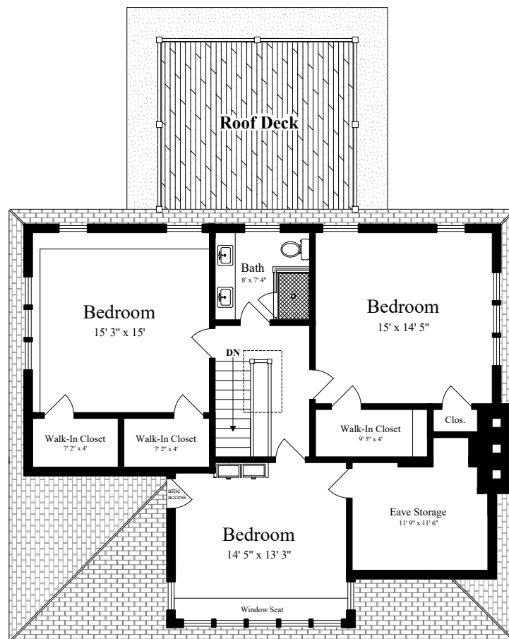
THIRD FLOOR (ceiling = 8' 9")
