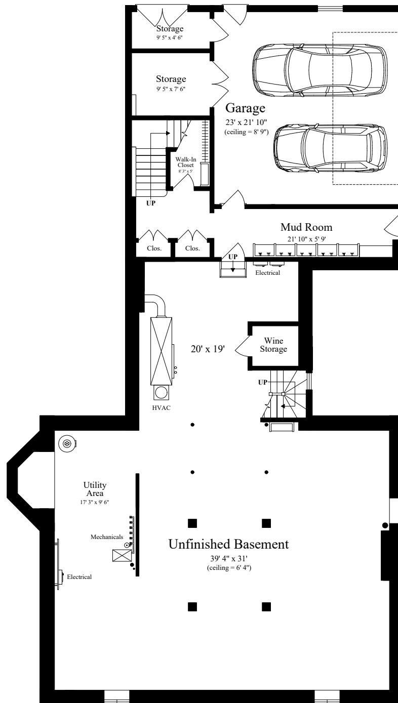
LOWER LEVEL (ceiling = 8')
