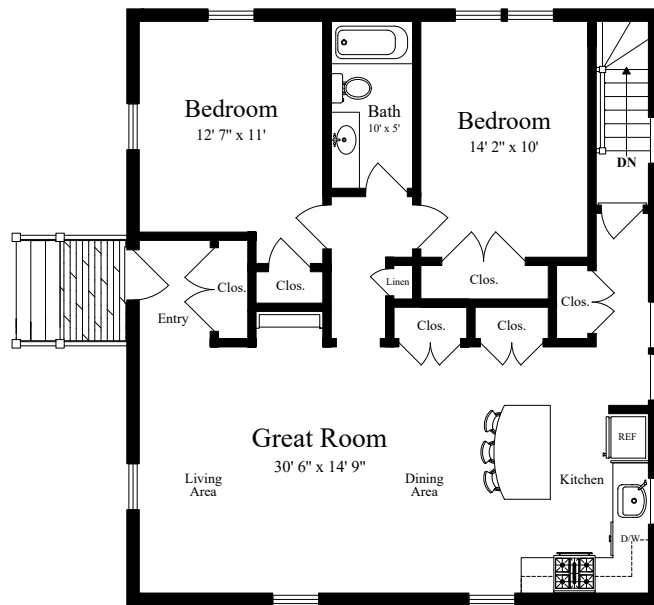
SECOND FLOOR Carriage House (ceiling = 8' 9")
