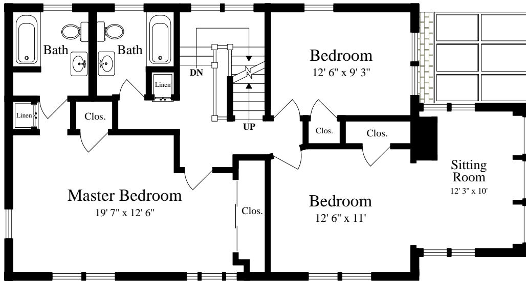
SECOND FLOOR (ceiling = 7' 10")
