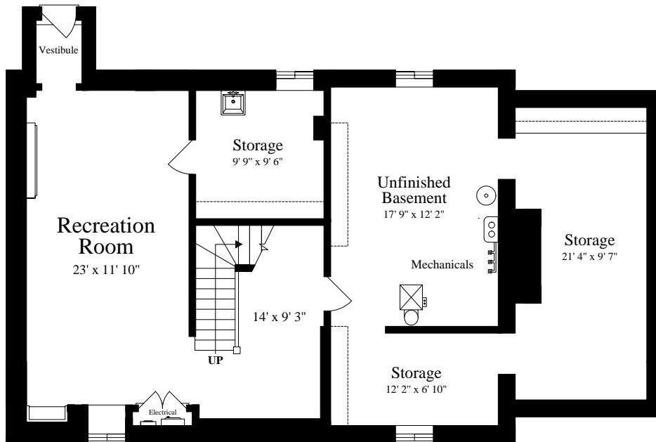
LOWER LEVEL (ceiling = 7' 4")
