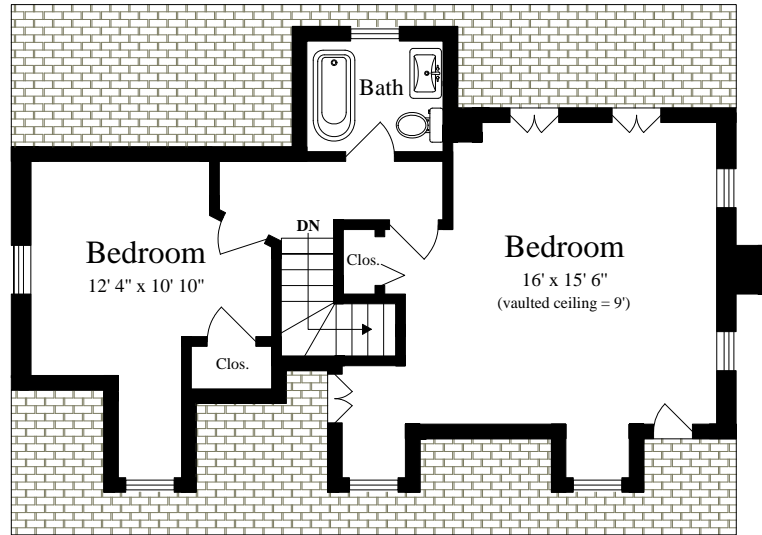
THIRD FLOOR (ceiling = 7' 3")
