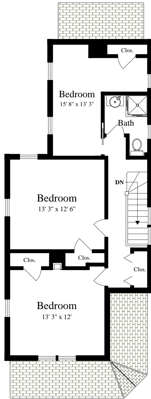
SECOND FLOOR (ceiling = 8')
