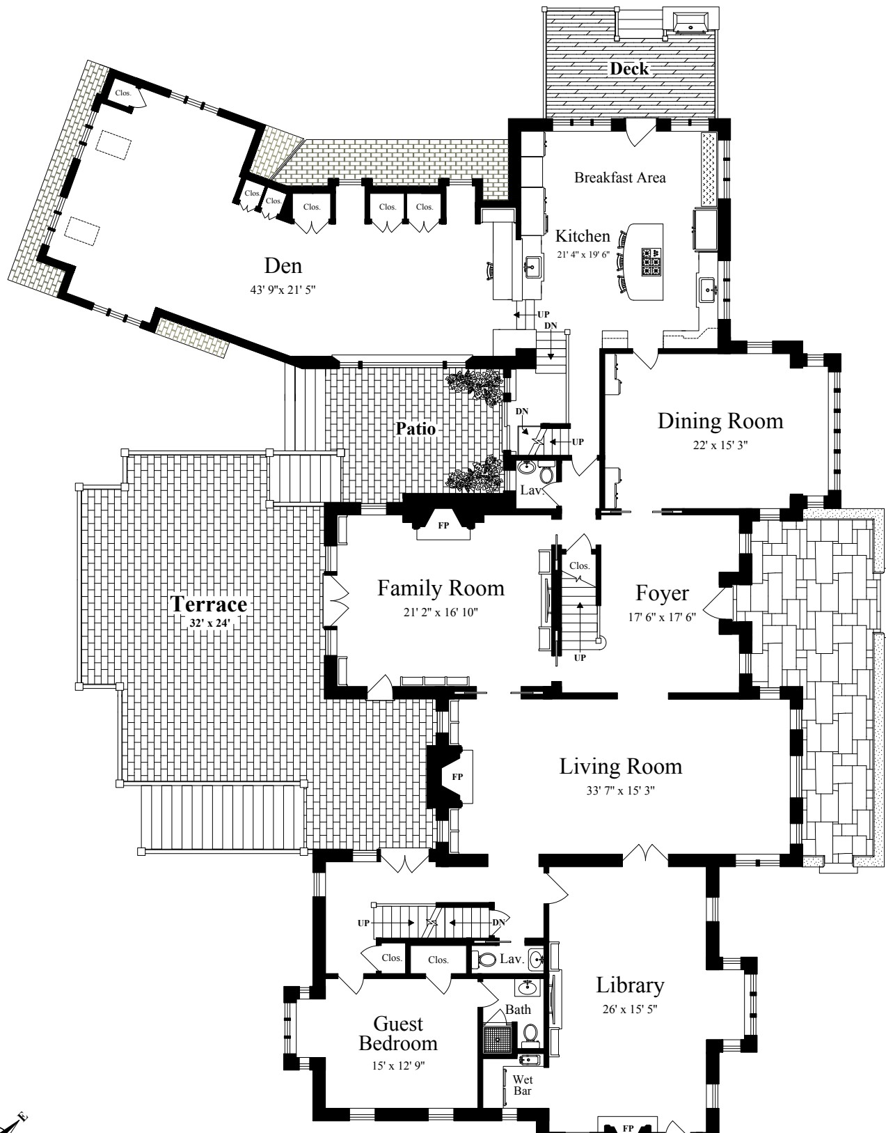
FIRST FLOOR (ceiling = 8')
