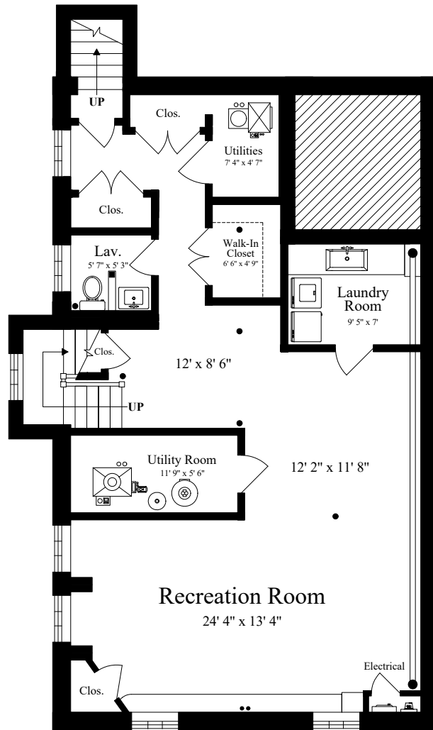
LOWER LEVEL (ceiling = 7')
